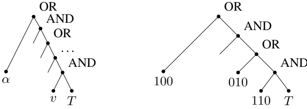
Figure 2: Deep pruning vs expected pruning.
