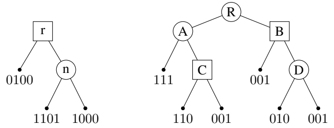
Figure 1: Two AND-OR DAGs with partially ordered values.
