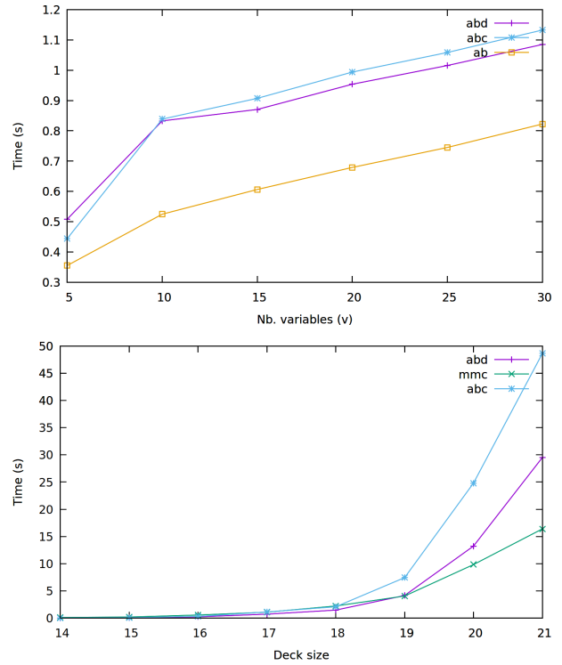
Figure 4: Experimental results on random (top) and racing (bottom). Top: d = 15 , b = 4 (varying v ), alternating DAGs, lattice 2^{2^S} . Bottom: h = 7 , g = 5 (varying d ), lattice 2^S .
