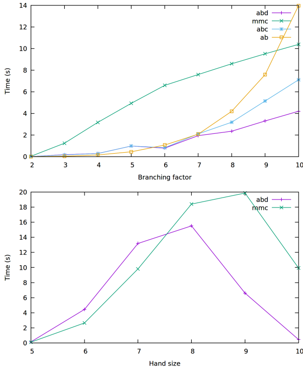
Figure 3: Experimental results on random (top) and racing (bottom). Top: d = 15 , v = 10 (varying b ), alternating DAGs. Bottom: d = 20 , g = 5 (varying h ). The lattice is 2^5 in both cases.
