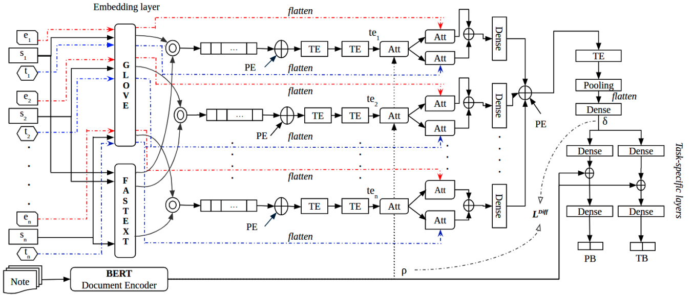
Figure 1: Architecture of the Temporal and Emotion-assisted Multitask Framework (TEMF). PE: positional encodings; TE: transformer encoder; Att: additive attention.
