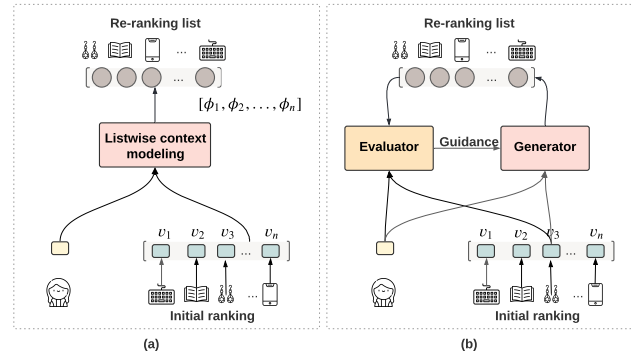
Figure 2: Re-ranking network architectures. (a) A typical neural re-ranking architecture for learning by observed signals. (b) The evaluator-generator paradigm for learning by counterfactual signals.
