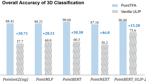
Figure 3: Overall Accuracy of 3D Classification (%) . Our method demonstrates a substantial improvement over vanilla frozen ULIP 3D backbones in classifying ModelNet40 downstream data.
