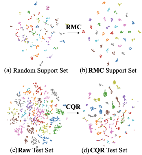
Figure 5: t-SNE of Random&amp;RMC support set, Raw&amp;CQR test set.
