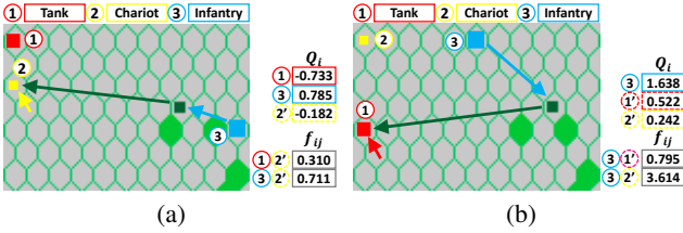
Figure 8: Visualization of evaluation for (a) MVD and (b) \text{NA}^2\text{Q} .
