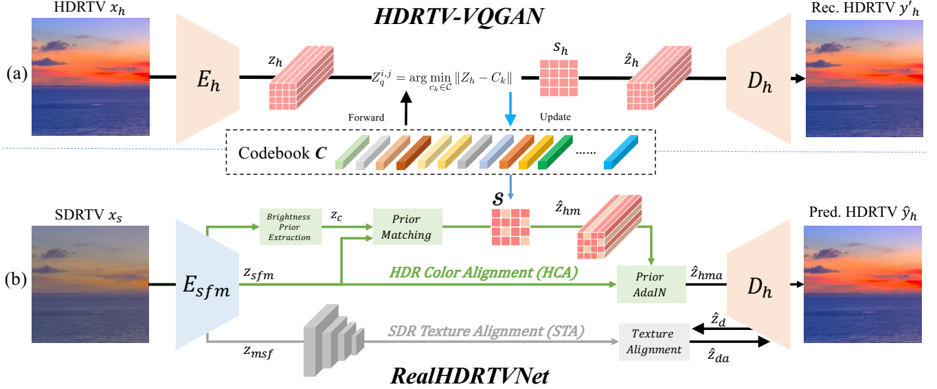
Figure 2: RealHDRTVNet framework. (a) HDRTV-VQGAN. We first pre-train an HDRTV-VQGAN to learn to store HDRTV priors through self-reconstruction. (b) RealHDRTVNet. The learning modulation encoder E_{sfm} obtains “nearly high-quality HDRTV features”. Next, the HDR Color Alignment HCA module aligns the input features with HDRTV in the color dynamic range dimension. In addition, the SDR Texture Alignment STA module is used to align the texture with the input SDRTV. This makes the dynamic range information of the conversion result consistent with HDRTV, and the texture details consistent with SDRTV.
