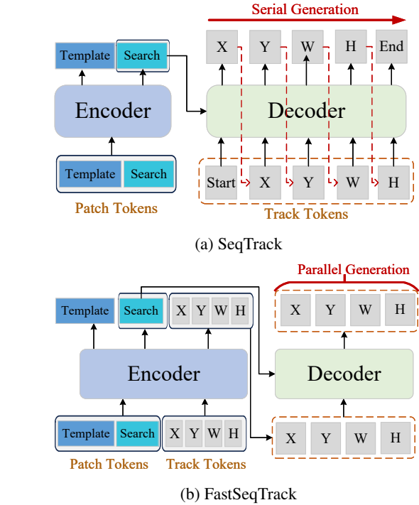
Figure 1: Comparison of tracking frameworks. (a) SeqTrack with a randomly initialized start token inferring in an auto-regressive sequence generation manner. (b) FastSeqTrack with initially guessed tracking tokens inferring in a one-pass sequence generation manner.
