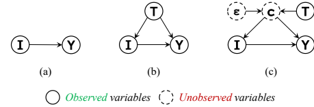
Figure 1: Conventional modeling versus a more rational modeling approach. (a) is the conventional modeling, (b) uses time as additional information where time acts as the confounder, and (c) is the rational modeling proposed in this work. I \rightarrow Item; Y \rightarrow User feedback; T \rightarrow Timestamp; \epsilon \rightarrow exogenous variables of confounders; c \rightarrow confounders.
