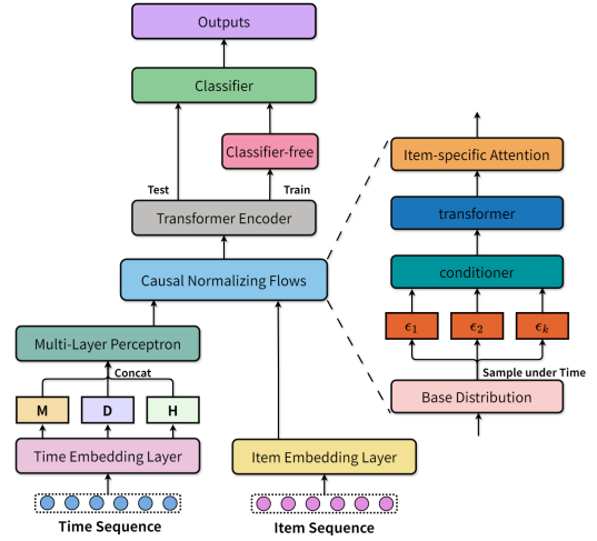
Figure 3: The architecture of our framework FCSRec.
