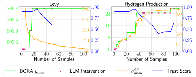
Figure 4: LLM intervention monitoring during a BORA run on 10D Levy (left) and Hydrogen Production (right). Mean uncertainty and Trust scores are also overlaid to highlight their interrelationships.
