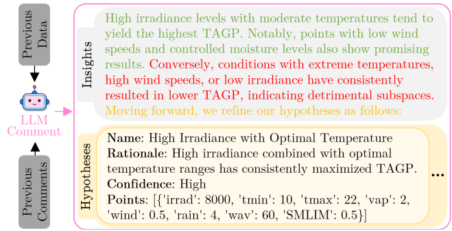
Figure 2: The LLM agent commenting and refining its hypotheses on the Sugar Beet Production experiment (complete comment in the SM). This experiment is detailed in Section 4.1.
