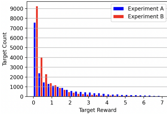
Figure 5: Target Reward Histograms (based on WLFV forecasts)
