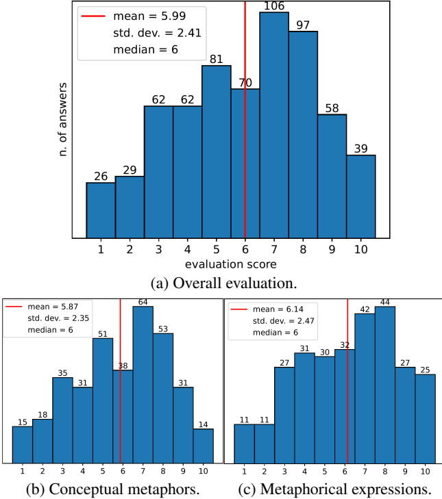
Figure 2: The overall results of the human evaluation (a) and a detailed breakdown for the combinations representing conceptual metaphors (b) and metaphorical expressions (c).
