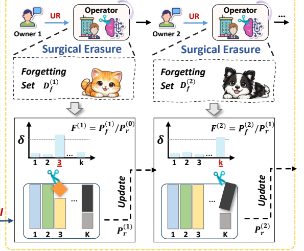
Figure 2: The pipeline of OTK that consists of two stages. In the first stage, the model provider (MP) performs one-turn post-training to construct a traceable and editable codebook-based proxy. In the second stage, the service operator (SO) handles unlearning requests locally by estimating the forget set’s token distribution and selectively updating the associated tokens to erase their influence.
