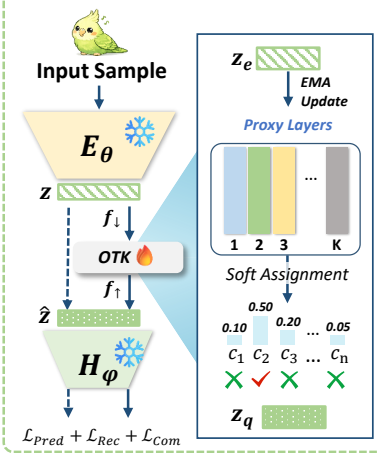
Figure 2: The pipeline of OTK that consists of two stages. In the first stage, the model provider (MP) performs one-turn post-training to construct a traceable and editable codebook-based proxy. In the second stage, the service operator (SO) handles unlearning requests locally by estimating the forget set’s token distribution and selectively updating the associated tokens to erase their influence.
