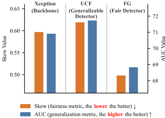
Figure 2: Illustration of the generalization–fairness trade-off in prior works. AUC and Skew [Geyik et al. , 2019] are reported on CDFv2, with all methods trained on FF++. UCF [Yan et al. , 2023] and FG [Lin et al. , 2024] adopt Xception [Chollet, 2017] as backbones.
