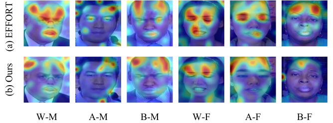
Figure 6: Attention heatmaps on samples from six demographic subgroups in DFDC. (a) EFFORT attends to demographic-correlated regions. (b) OSD highlights forgery-related regions (e.g., blending boundaries) rather than demographic-specific facial features.
