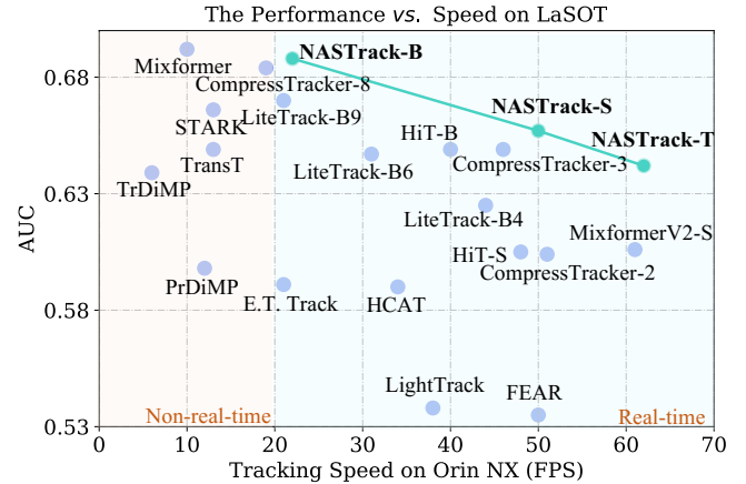
Figure 1: Performance comparisons with state-of-the-art trackers in terms of AUC and speed on LaSOT. The proposed NASTrack is superior to LiteTrack and CompressTracker family [Wei et al. , 2024a; Hong et al. , 2025], while achieving faster speed on Jetson Orin NX. Best viewed in color.
