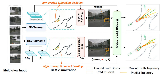
Figure 1: Illustration of the difference between existing vision-based methods (top) and our approach (bottom). Our method leverages BEVFormer++ to explicitly predict dynamic motion parameters—including velocity, acceleration, and heading angle—which are used to enhance BEV feature generation and trajectory prediction.
