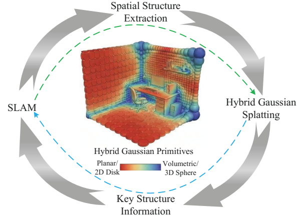
Figure 1: The tightly coupled framework of GGF-SLAM. The solid gray cycle demonstrates our proposed bidirectional mutual enhancement between SLAM and Hybrid Gaussian Splatting, effectively bridging the gap present in existing unidirectional or loosely coupled frameworks (dashed arrows).
