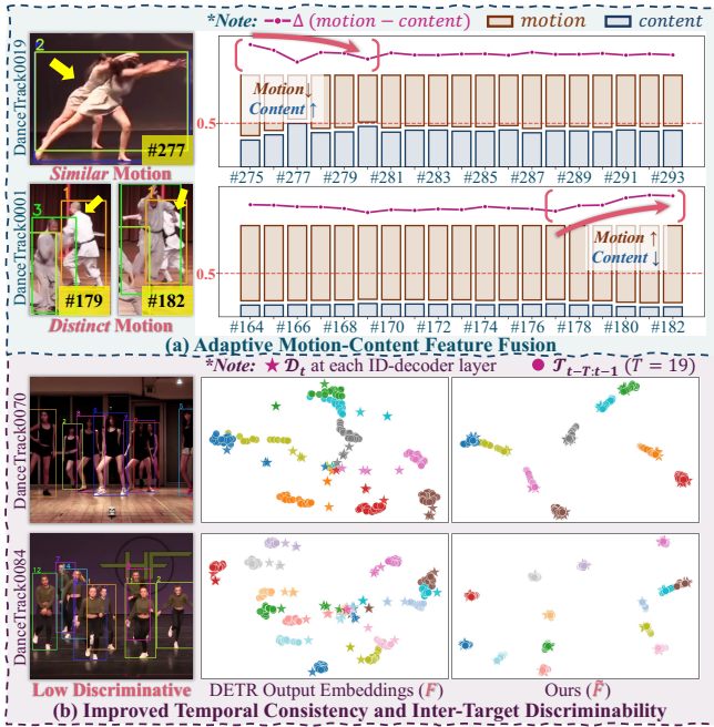
Figure 3: Visualization of motion-aware target representations. The points are visualized with t-SNE, and points with the same color correspond to the same identity.
