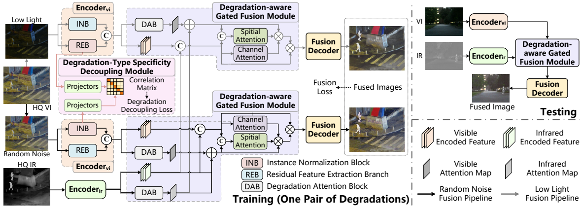
Figure 3: The structure detail of Specifuse. For clarity of demonstration, we only show the fusion pipeline of visible low-light and noise degradation in the training phase.
