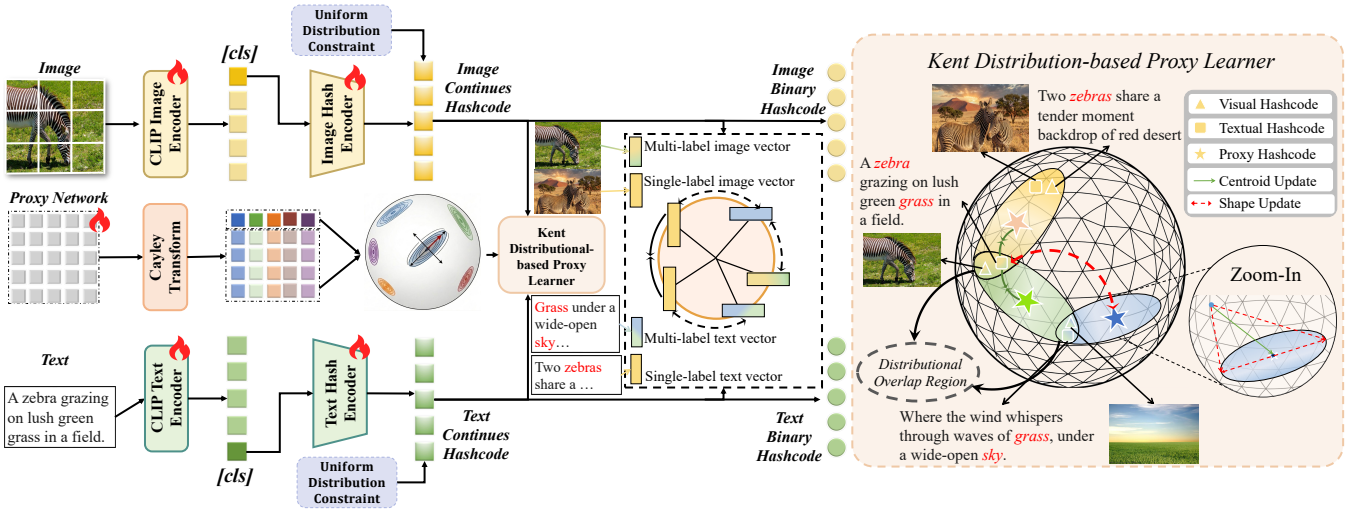
Figure 2: Overview of the Kent-based Distributed Proxy Hashing (KDPH) framework. It consists of a CLIP-based feature extraction module and a Kent-based Distributional Proxy Learner. As shown in the right panel, we model class proxies as learnable anisotropic distributions rather than static points. Through the gradient decoupling mechanism by separating centroid \mu and variance B, \Gamma , the model dynamically stretches the proxy’s semantic volume to accommodate multi-label variance, effectively mitigating proxy collapse and oscillation.
