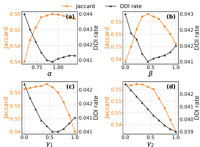
Figure 4: Hyperparameter test on the MIMIC-III dataset. (a) Reconstruction weight, (b) KL regularization weight, (c) Representation-level DDI regularization weight, (d) Generation-level safety regularization weight.
