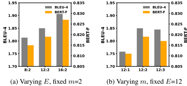
Figure 6: Explanation quality under varying interaction sparsity.
