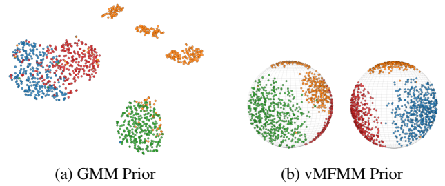
Figure 4: t-SNE visualization of latent representations on Amazon.
