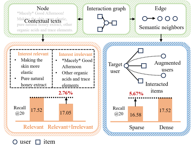
Figure 1: The motivation of data enhancement with contextual texts and semantic neighbors.
