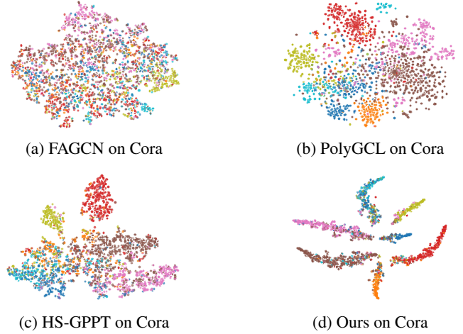
Figure 5: Comparative 1-shot learning scatter plots on the Cora dataset. (a) FAGCN; (b) PolyGCL; (c) HS-GPPT; (d) Ours.
