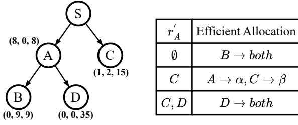
Figure 1: An example illustrating the failure of single-parameter monotonicity conditions in the combinatorial setting.
