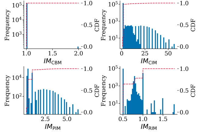
Figure 1: Distribution of tuple inconsistency measures.
