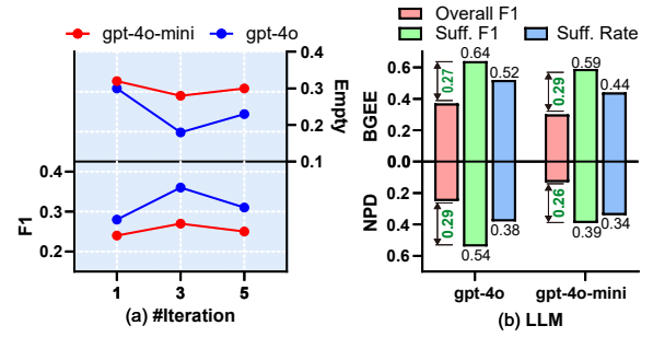
Figure 3: (a) Iteration count impact on BGEE. (b) F1 for all queries vs. a_i = \text{SUFFICIENT} queries.
