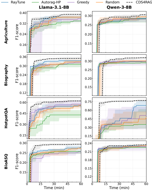
Figure 5: Optimization trajectories of CDS4RAG against the state-of-the-art algorithms for RAG over 10 runs
