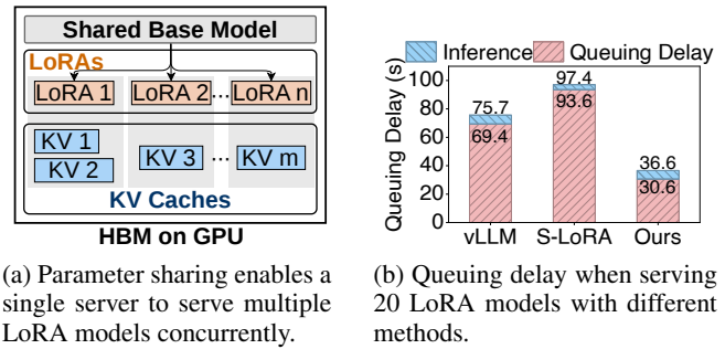
Figure 1: Existing multi-LoRA serving methods and their bottleneck.
