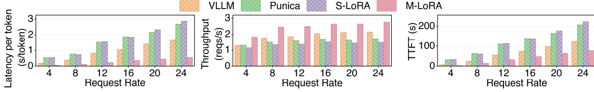
Figure 7: Latency per token, throughput, and TTFT for different systems serving LLaMA-2-13B on an A100 GPU.
