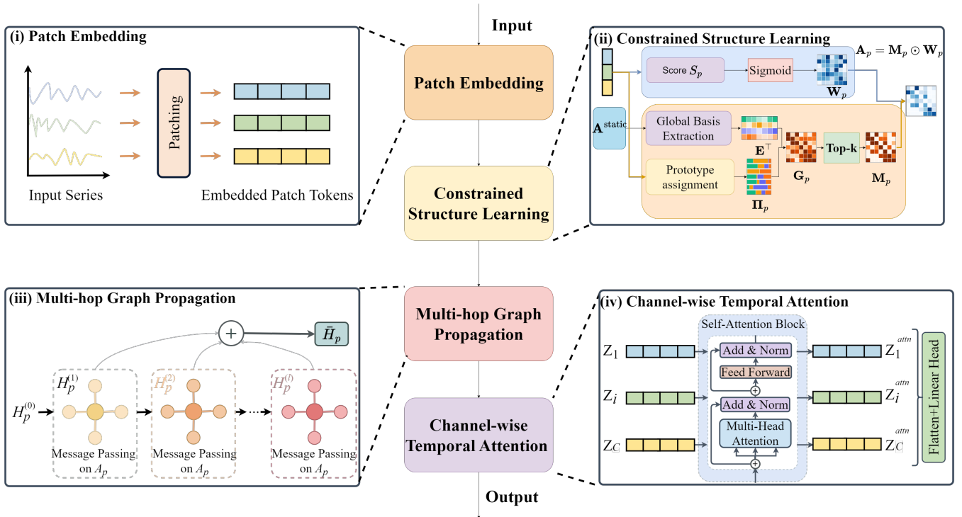
Figure 2: The overall architecture of ConDyGNet.
