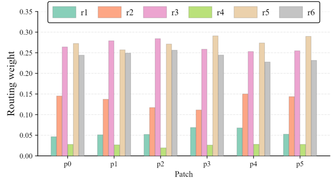
Figure 4: Visualization of patch-wise basis routing weights on a representative Weather sample ( L=96 , patch length 16, R=6 ). Each group corresponds to a patch, and each bar denotes the channel-averaged routing weight of a basis mode.
