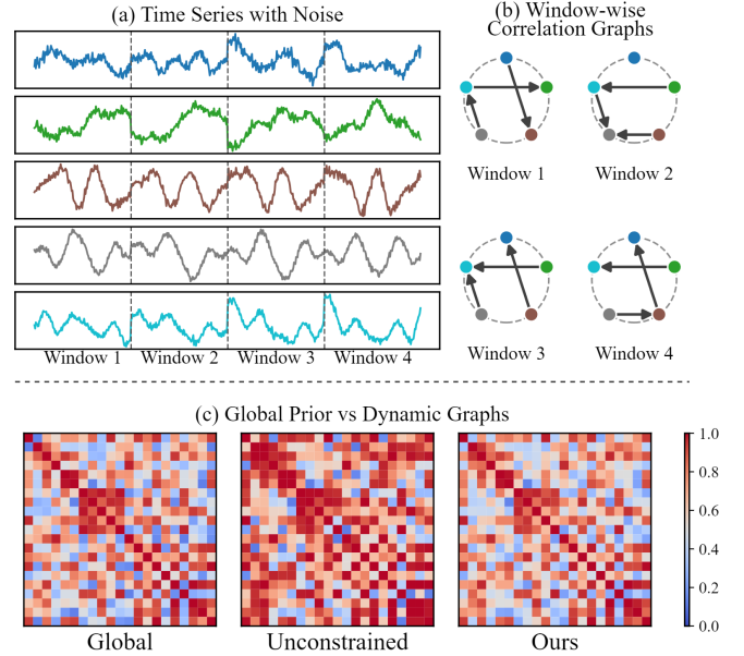
Figure 1: (a) Multiple variables change with the window size. (b) The relationships between variables change over time windows; in each window, we only show the three strongest relationships. This demonstrates that the relationships between channels are dynamic. (c) In a representative window, we compared the global matrix, the unconstrained matrix, and our proposed structure. As can be seen in the figure, the structure generated by our method is closer to the global matrix, while the unconstrained method exhibits more noise. This demonstrates the importance of structural constraints.
