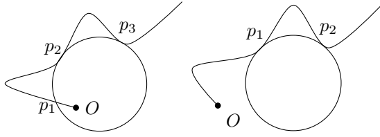
Figure 1: In \mathbb{R}^4 (left), the 3-sphere that goes through the points p_1, p_2, p_3 on the moment curve and is tangent to the moment curve on p_2 and p_3 , has no other intersections with the moment curve after the origin. In \mathbb{R}^3 (right), the sphere that is tangent to the moment curve on p_1 and p_2 has no other intersections with the moment curve.
