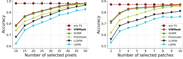
Figure 3: Classification accuracy on MNIST and Fashion-MNIST as a function of the mean number of selected pixels or patches. w/o FS (using all features) achieves the highest accuracy, while VIBMask consistently delivers strong performance with more efficient feature selection, particularly when very few pixels or patches are selected.
