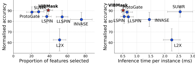
Figure 2: Normalized performance of selector-predictor IWFS methods. Left: trade-off between feature proportion and accuracy, showing sparsity-accuracy balance. Right: inference time vs. accuracy, indicating efficiency. VIBMask consistently achieves high accuracy with fewer features and low latency, balancing interpretability and efficiency.
