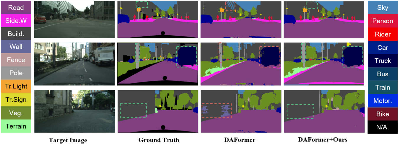
Figure 3: Qualitative comparisons on the GTA \rightarrow Cityscapes benchmark. We compare the segmentation maps generated by the baseline DAFormer and our method. Red dashed boxes highlight failure cases in the baseline predictions, while green dashed boxes demonstrate that our method successfully corrects these errors, yielding predictions that are well-aligned with the Ground Truth.
