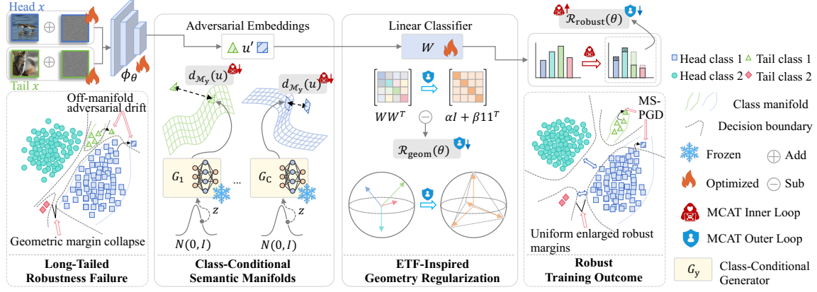
Figure 2: Overview of MCAT for long-tailed adversarial robustness. Left: Under long-tailed data, standard adversarial training exhibits (i) off-manifold adversarial drift and (ii) geometric margin collapse for tail classes. Middle: MCAT couples two mechanisms: a class-conditional manifold distance penalty in feature space and an ETF-inspired geometric alignment of classifier weights. Right: Manifold-Constrained PGD (MS-PGD) learns robust decision boundaries near high-density semantic support while preserving enlarged (and more uniform) robust margins across classes.
