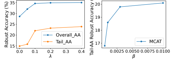
(a) Robustness vs. \lambda . (b) Tail robustness vs. \beta .
