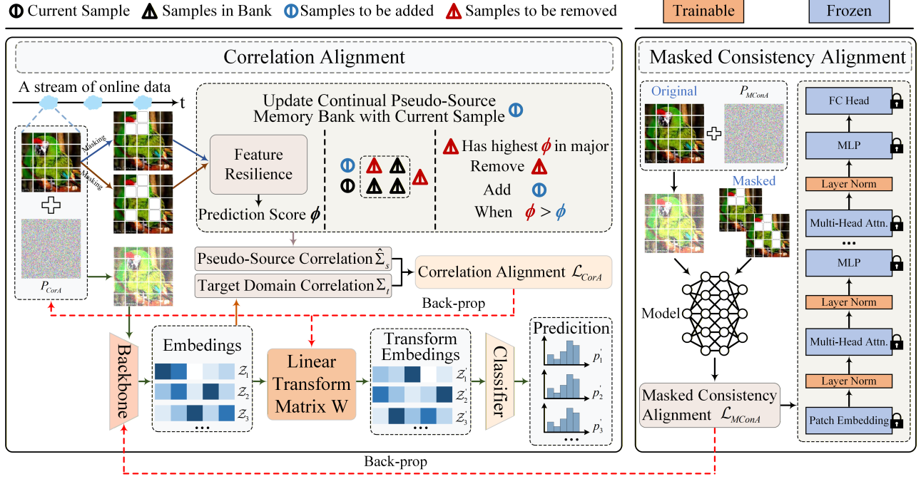
Figure 1: The framework of D-Align.
