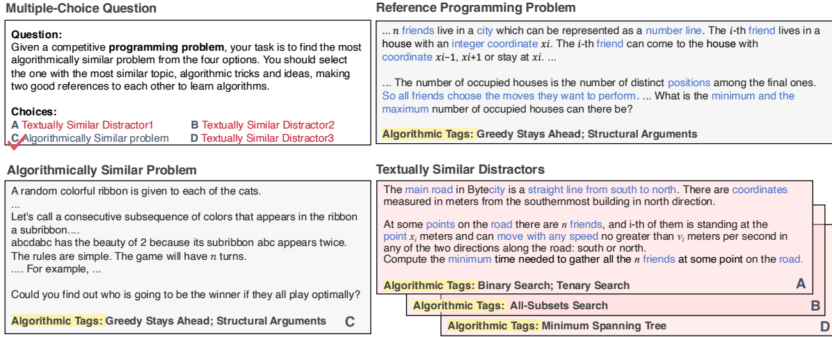
Figure 1: An example from AlgoSimBench, with one algorithmically similar problem and a textually similar distractor as an example. The blue-highlighted text makes the reference problem and the distractor look similar.
