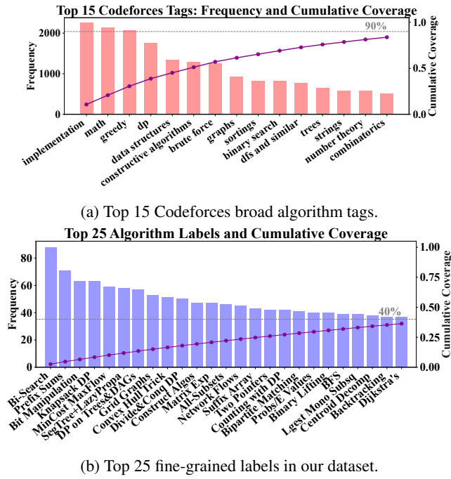
Figure 2: Comparison between Codeforces tag distribution and our fine-grained tag distribution.
