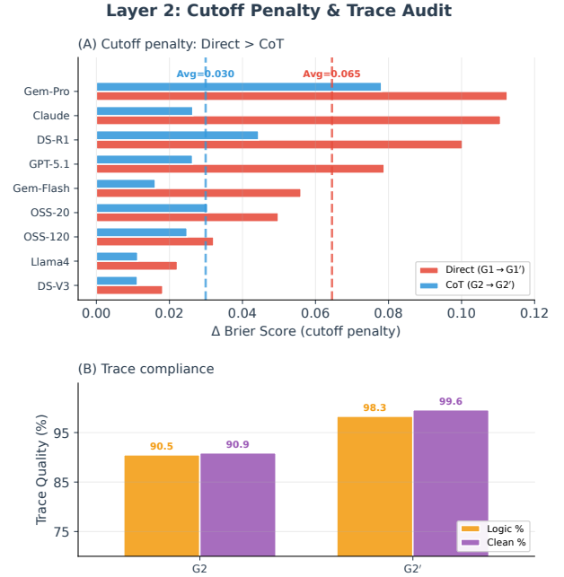
Figure 4: Layer 2: Trace compliance. (A) Cutoff penalty on Pre-cutoff is larger for direct prompting than CoT. (B) Trace audit metrics improve from G2 to G2' .
