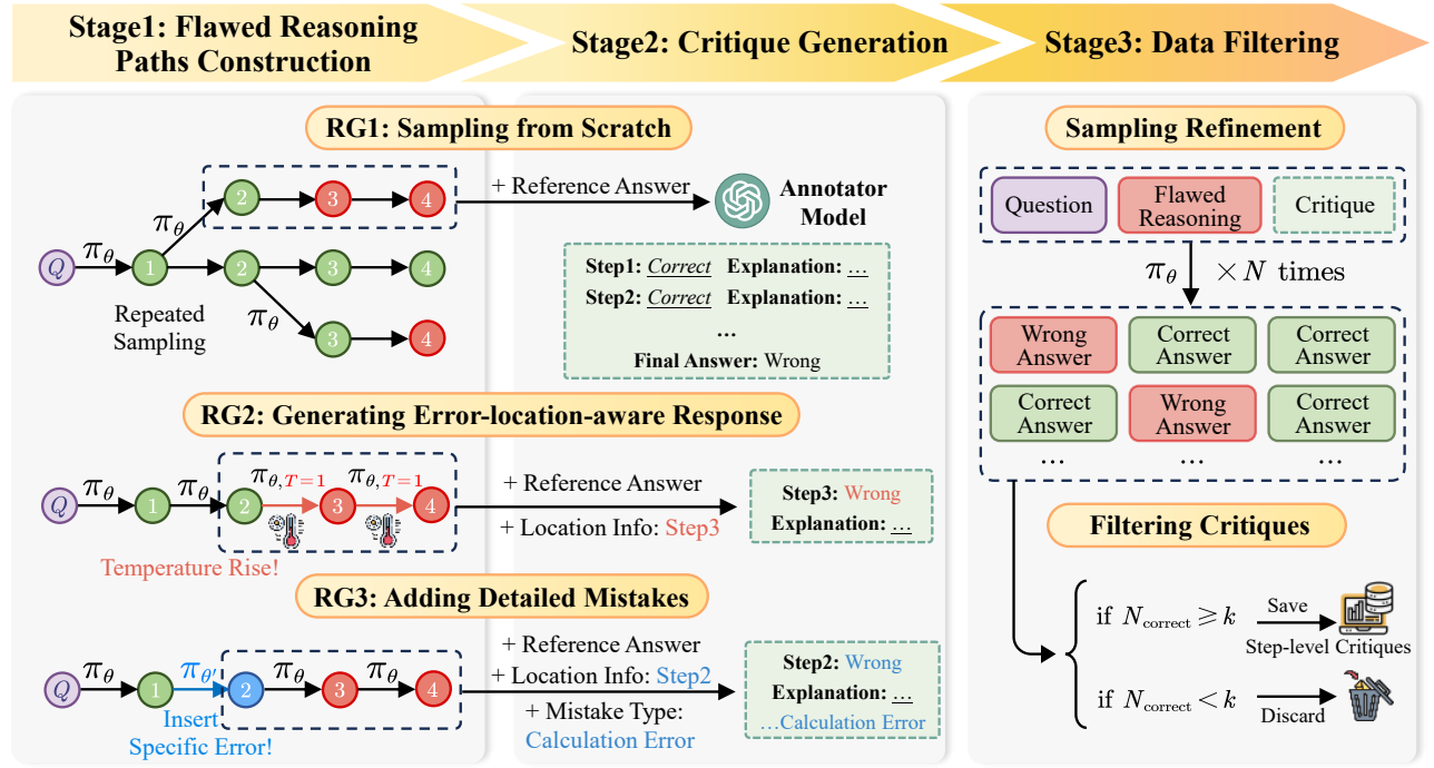
Figure 1: The overview of AutoMathCritique framework.
