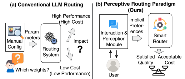
Figure 1: Perceptive LLM routing paradigm.
