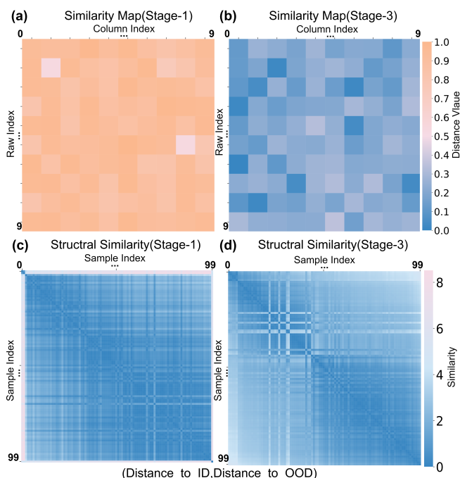
Figure 5: Analysis of structural distribution consistency. (a) (b) Similarity maps between generated molecules and guidance graphs. (c) (d) Sample \times Sample structural similarity matrices.
