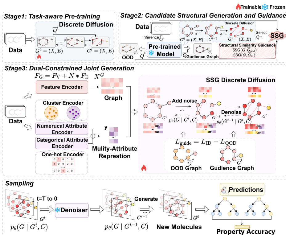
Figure 1: Overview of the proposed D 2 G-TO framework.
