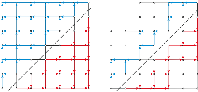
Figure 2: Comparison of the global redistancing algorithm on a dense grid (on the left) with the local redistancing (on the right) for SBS; bricks are 3 \times 3 distances in size. The dots represent the distance values. Red and blue dots are the distances outside and inside the object, respectively. The dashed line represents the surface, set by distances colored white. Arrows show the order of updating the values. Local redistancing ignores the bricks without the surface (grey).
